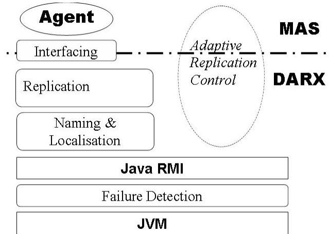
Figure 1. DARX framework design.
