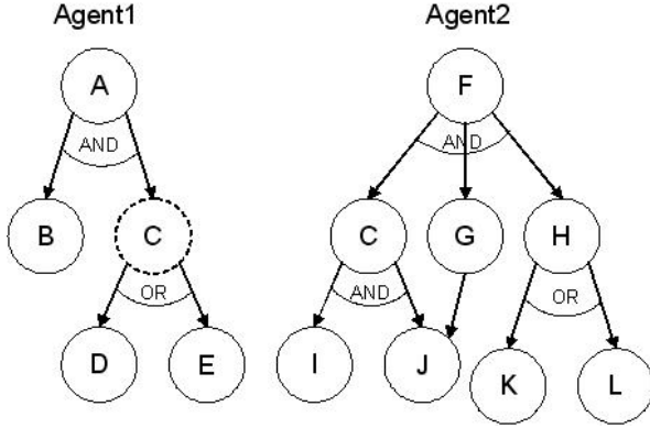
Figure 3. Example of plans of two interacting agents.
