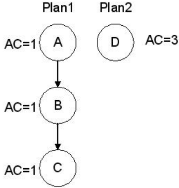
Figure 4. Impact of time in the criticality of actions.
