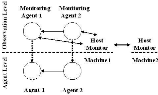
Figure 2. Architecture for replication control.
