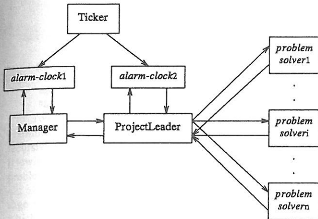
Figure 10. A Scheme for Distributed Problem Solving
